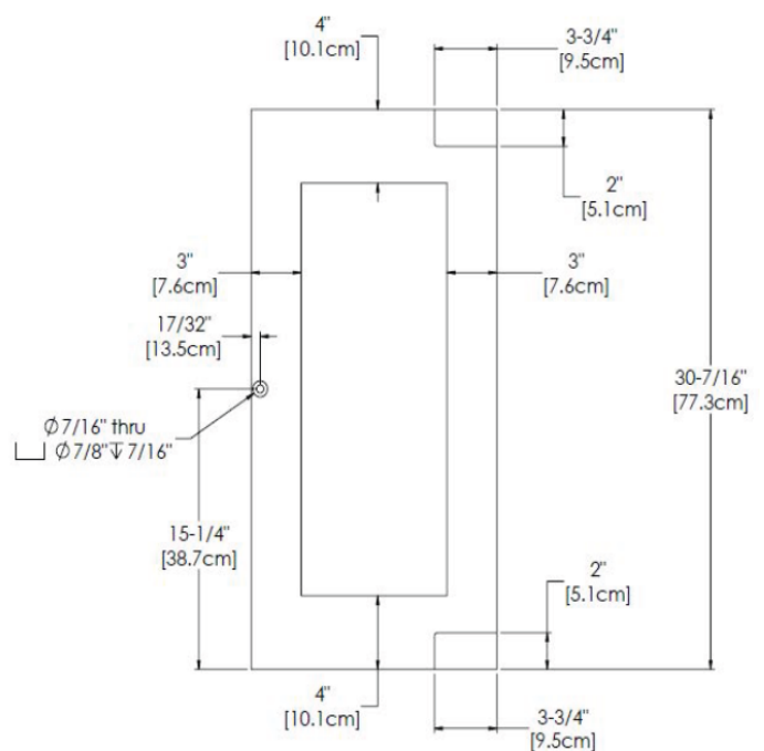
Right Hand Hinged Door 15" (38.1 cm) wide appliance
